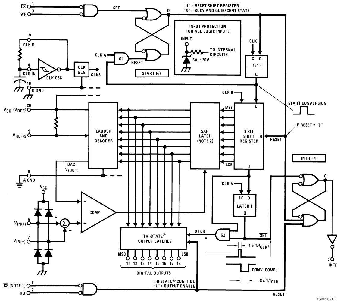
FIGURE 4. Block Diagram
