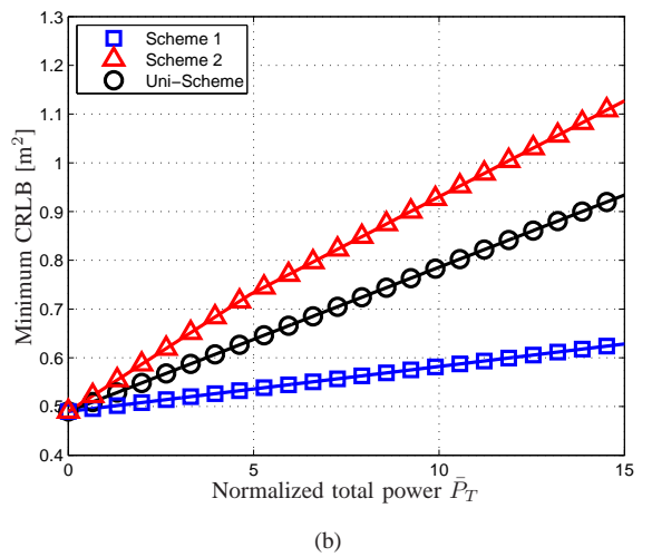
Fig. 5. Comparison of different schemes for power allocation in terms of (a) average CRLB, (b) minimum CRLB for the scenario in Fig. 4.
