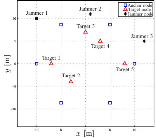
Fig. 7. The network considered in the simulations, where the anchor node positions are [-10 \ 0] , [-5 \ -5\sqrt{3}] , [-5 \ 5\sqrt{3}] , [5 \ 5\sqrt{3}] , [5 \ -5\sqrt{3}] , and [10 \ 0] m., the target node positions are [-7 \ 0] , [-3 \ -4] , [0 \ 7] , [3 \ 5] and [8 \ 0] m., and the jammer node positions are [-10 \ 10] , [1 \ 11] , and [12 \ 5] m.
