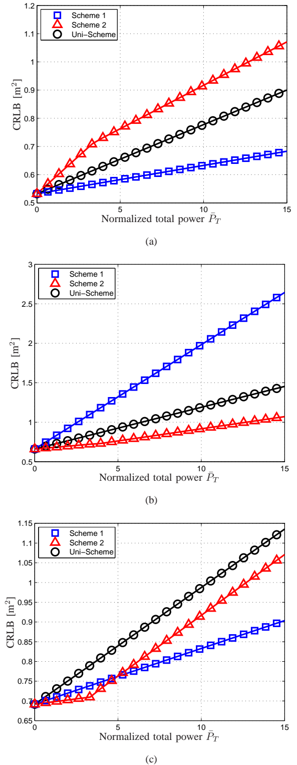
Fig. 3. CRLBs for different schemes of power allocation for (a) Target 1, (b) Target 2, and (c) Target 3 (for the scenario in Fig. 1).
