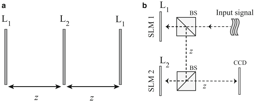
Fig. 6.6 (a) Optical system for the FRT using three generalized lenses separated by distance z . (b) Experimental implementation of a programmable optical FRT setup: two reflective phase-only SLMs are used to realize the generalized lenses L_1 and L_2 . The output signal is registered by a CCD camera in real time [33]
