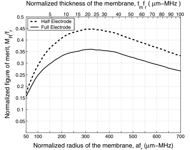
Fig. 7. Normalized gain-bandwidth product as a function of normalized membrane radius or thickness for receiver cMUTs with full metallized (solid), or half metallized membranes (dashed). The curves are independent of t_g . C_S=0 .
