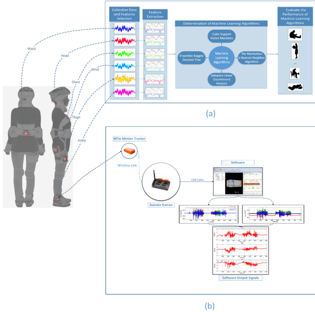
Fig. 1. a) Flowchart of activity recognition. b) The system consisting of MTw sensors and the Awinda station on the body, working phases, and signal acquisition.
