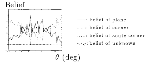
Figure 9: Belief assignment to a plane at r = 50 cm scanned with the Panasonic sensing unit.
