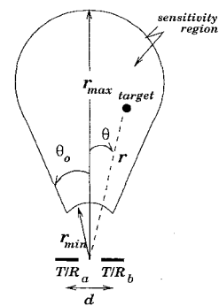
Figure 1: Sensitivity region of an ultrasonic transducer.
