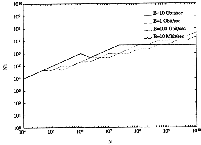
Figure 11.20: N_1 versus N for (R2d, OPl) II. p = 0.8 , f = 200 , E_o = 100 pJ.
