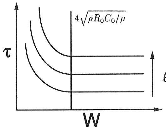
Figure 5.3: Repeated interconnection model .
