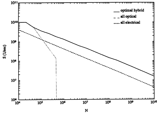
Figure 11.17: S versus N for (N2d, OPl) III. B = 100 Mbit/sec, p = 0.8 , f = 200 , E_o = 100 pJ.
