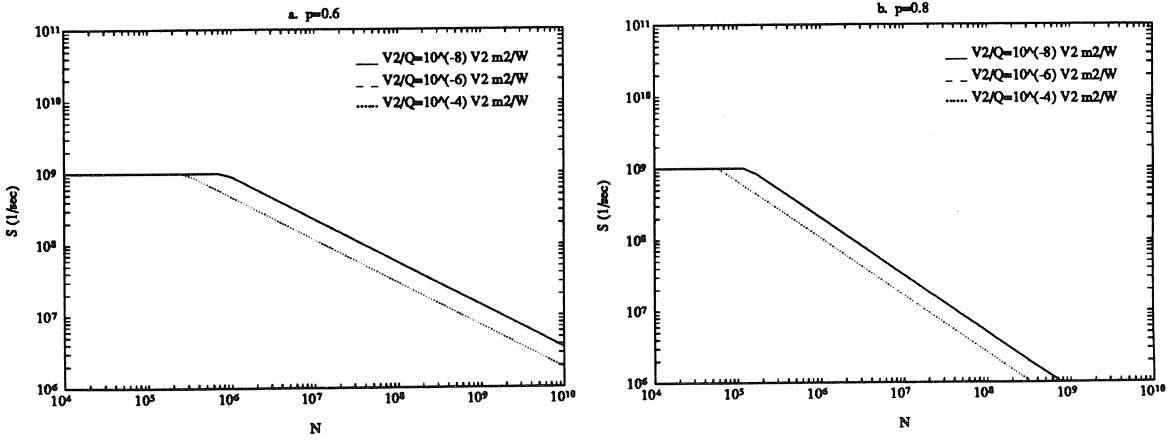
Figure 10.14: S versus N for B = 1 Gbit/sec for repeaters in 2 dimensions. We take k = 5 , M = 10 and T = R_0 C_0 = 1 nsec so that \chi = 1 . d_d is assumed to be small enough to have no effect. The curves corresponding to the two smaller values of V^2/Q overlap.
