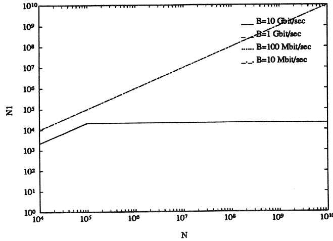
Figure 11.11: N_1 versus N for (R2d, O2d) . p = 0.8 , f = 2 , E_o = 1 pJ.
