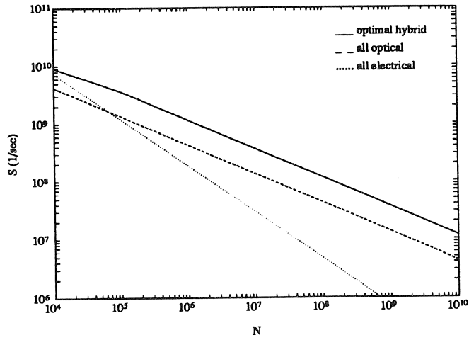
Figure 11.19: S versus N for (R2d, OPl) I. B = 10 Gbit/sec, p = 0.8 , f = 2 , E_o = 1 pJ.
