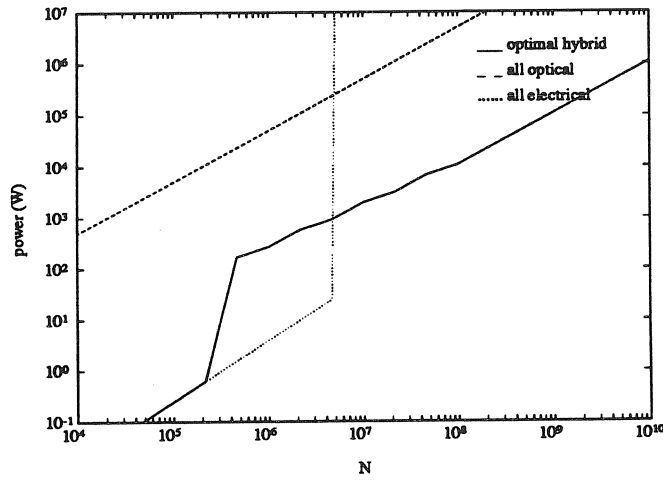
Figure 11.9: \mathcal{P} versus N for (N2d, O2d) . B = 100 Mbit/sec, p = 0.6 , f = 2 , E_o = 100 pJ.
