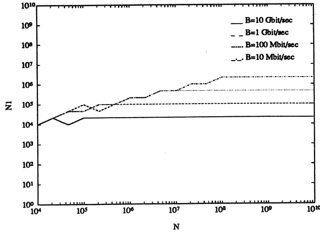
Figure 11.10: N_1 versus N for (N2d, O2d) IV. p = 0.8 , f = 2 , E_o = 100 pJ.
