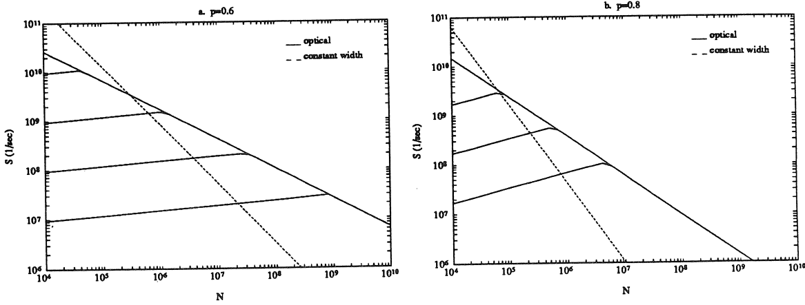
Figure 10.8: Comparison of optical and normally conducting interconnections for same values of B . Similar parameter values are taken as in the previous figure. E/Q ranges from 10^{-21} \text{ m}^2 \text{ sec} to 10^{-13} \text{ m}^2 \text{ sec} in increments of 10^{-2} \text{ m}^2 \text{ sec} .
