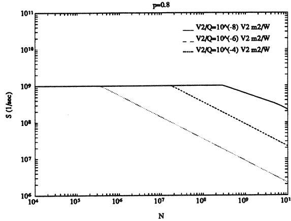
Figure 10.15: S versus N for B = 1 Gbit/sec for repeaters in 3 dimensions. We take k = 5 , p = 0.8 and T = R_0 C_0 = 1 nsec so that \chi = 1 . d_d is assumed to be small enough to have no effect.
