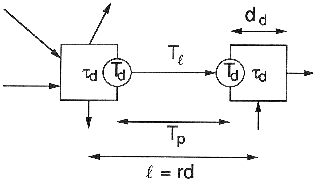
Figure 4.2: Factors determining the speed of the system. Two elements (graph nodes) sharing an (inter)connection (graph edge) of length \ell are shown. \tau_d is the time which elapses between arrival of new input to an element and updating of the output values. T is the minimum temporal pulse width. T_p is the propagation delay along the interconnection.
