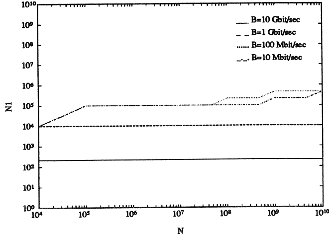
Figure 11.12: N_1 versus N for (N2d, OPl) I. p = 0.6 , f = 2 , E_o = 1 pJ.
