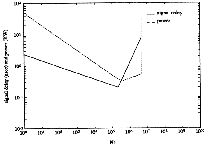
Figure 11.26: \tau and \mathcal{P} versus N_1 for (N2d, OPl) . N = 10^8 , B = 100 Mbit/sec, p = 0.6 , f = 2 , E_o = 1 pJ.
