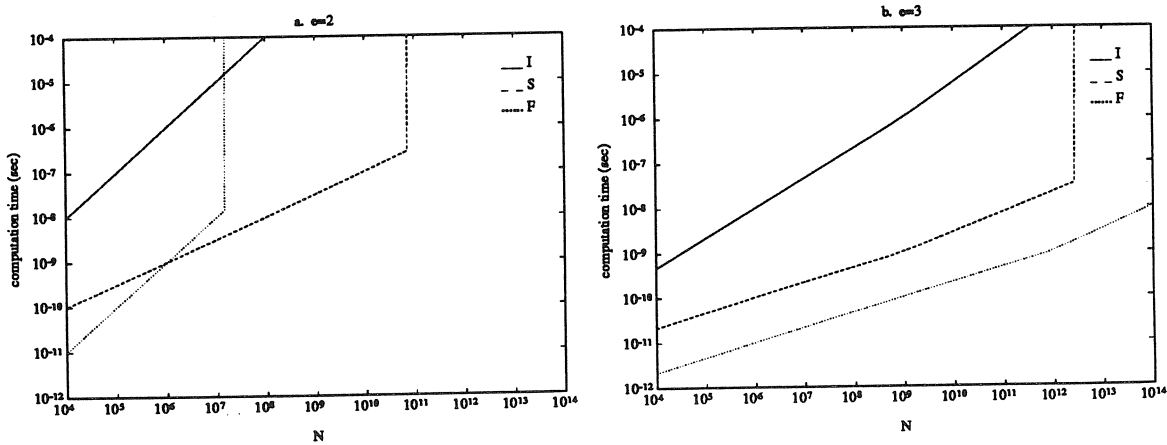
Figure 14.2: Computation time for the three methods with n_f = N^{2/e} for isomorphic simulation. \tau_d = 1 psec, \tau_o = 1 fsec, \tau_Q = 0.1 psec and d_d = 1 \mu\text{m} . The curves are terminated when the system linear extent exceeds 10 m.
