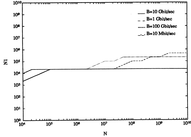
Figure 11.18: N_1 versus N for (R2d, OPl) I. p = 0.8 , f = 2 , E_o = 1 pJ.
