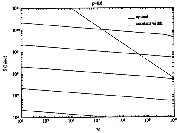
Figure 10.11: Comparison of optical and normally conducting interconnections for same values of B in 3 dimensions. Similar assumptions as in the previous figure are made. E/Q varies from 10^{-21} \text{ m}^2 \text{ sec} to 10^{-13} \text{ m}^2 \text{ sec} in increments of 10^{-2} \text{ m}^2 \text{ sec} .
