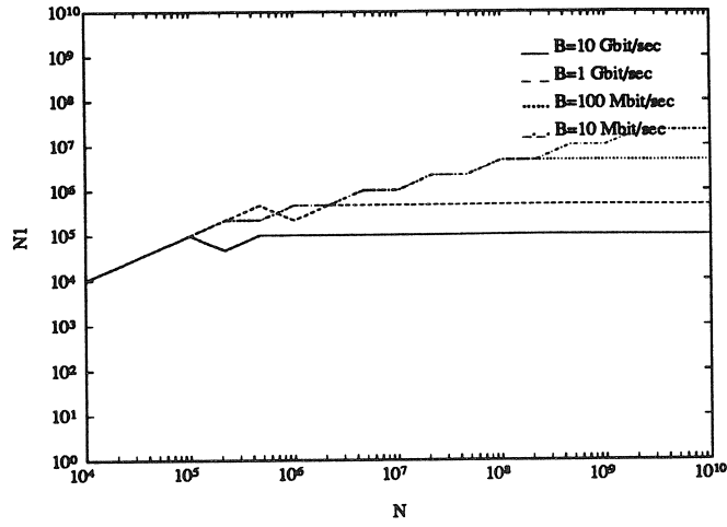
Figure 11.8: N_1 versus N for (N2d, O2d) III. p = 0.6 , f = 2 , E_o = 100 pJ.
