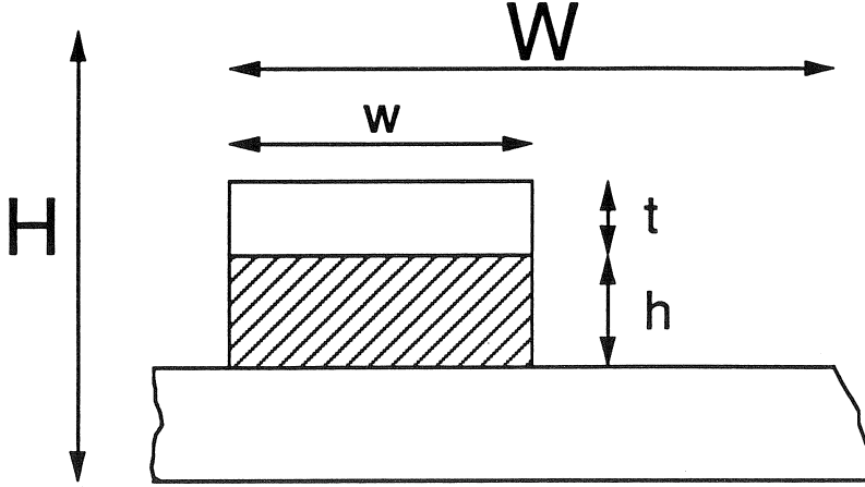
Figure 5.6: Physical cross section of interconnection model. t and h are the heights of the conductor and dielectric respectively. We constrain t \leq h and h \leq w/2 . These constraints not only ensure reasonable confinement of the fields, but also justify approximate use of a parallel plate model for calculating capacitances and inductances. W = 2w is the two dimensional minimum packing dimension. A = WH = 4w(h+t) \simeq 4w \max(h, t) = 4wh is the three dimensional minimum packing area.
