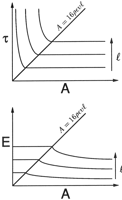
Figure 5.2: Normally conducting interconnection model when T_d \leq T_\ell .
