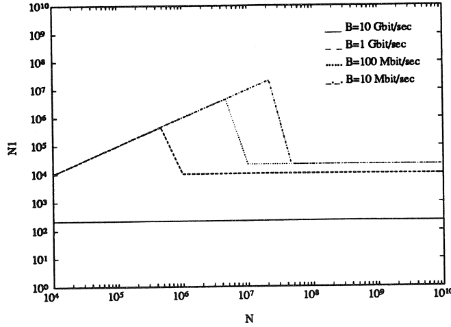
Figure 11.23: N_1 versus N for (N2d, O2d) V. p = 0.6 , f = 2 , E_o = 1 pJ.
