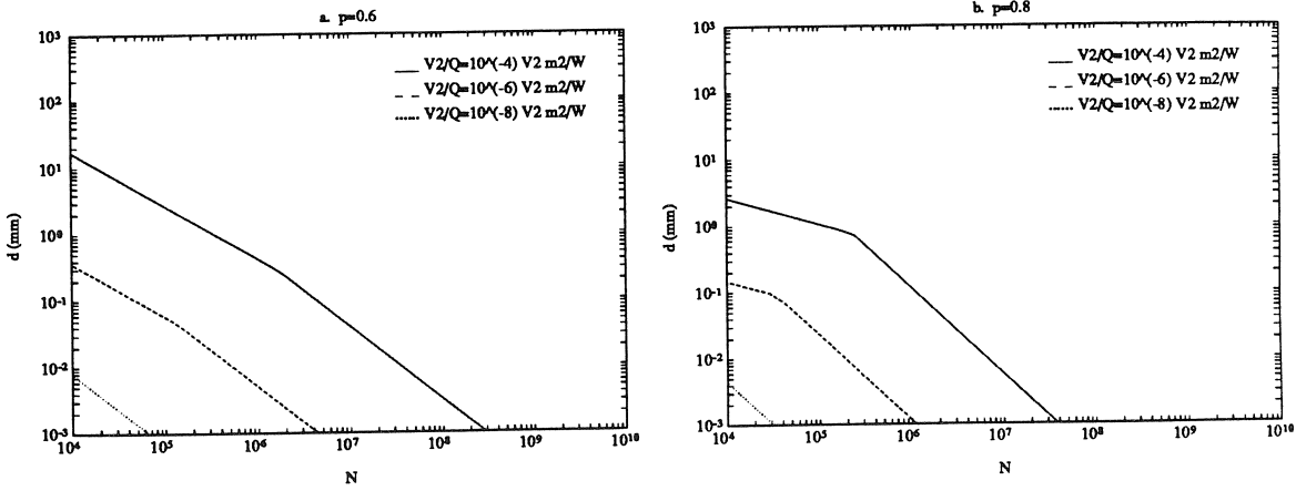
Figure 10.9: Cell size as set by heat removal. B is set to its largest possible value. We take k = 5 , M = 10 and assume that T_d is negligibly small.
