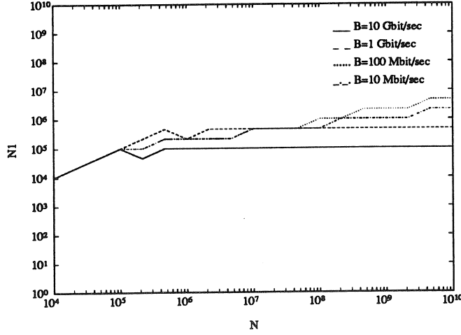
Figure 11.14: N_1 versus N for (N2d, OPl) II. p = 0.6 , f = 200 , E_o = 100 pJ.
