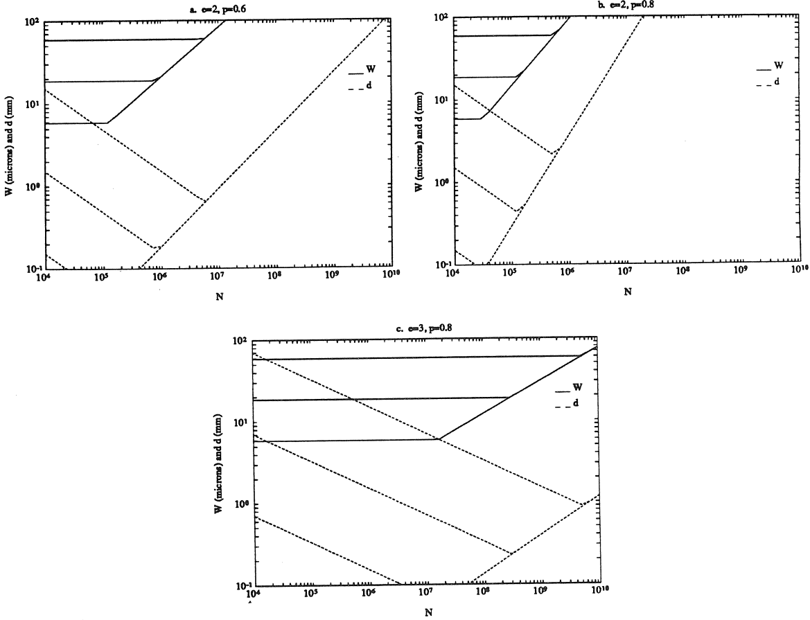
Figure 10.6: Critical width and cell size below which inductive effects need not be considered. Each part of this figure corresponds to those of the previous figure.
