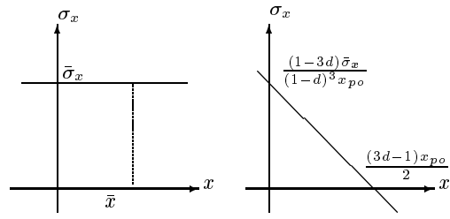
Figure 2: (a) Wigner distribution of the original exponential. (b) Wigner distribution of the approximate perspective projection: a chirp.
