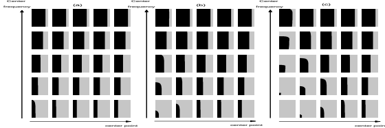
Figure 5: The dark regions represent the parameter combinations whose normalized error is less than 10%. See text for explanation.
